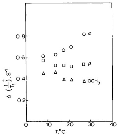
Fig.3. Plot of relaxation rate of protons of 4-MeOPy vs temperature. [P-450] = 2.3 \times 10^{-5} M, [4-MeOPy] = 15 mM, 0.1 M KPi in D 2 O, pH obs 7.5.
