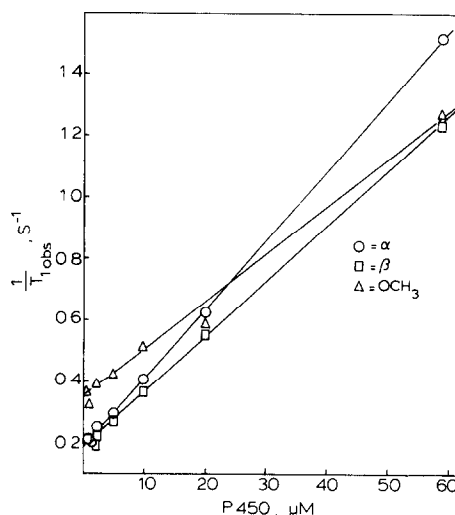
Fig.1. Plot of the rate of longitudinal relaxation of protons of 4-MeOPy vs concentration of P-450. 0.1 M \text{KPi} in \text{D}_2\text{O} , \text{pH}_{\text{obs}} 7.5 , 21^\circ\text{C} ; [4\text{-MeOPy}] = 6.7 \text{ mM} .
